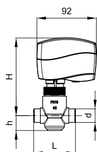
AMV(E) 130/140 + VZ 2
