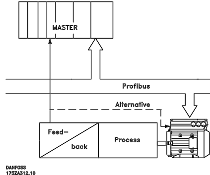
Closing the control loop outside the fieldbus for extremely fast feed-back
